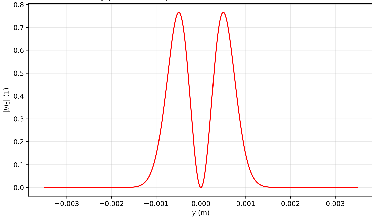
Intensity profile I(x=0, y, z=0.159)/I_0 , P_{in}=0.5P_{cr} , artificial time
